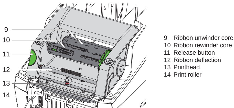
Figure 2 Print module
