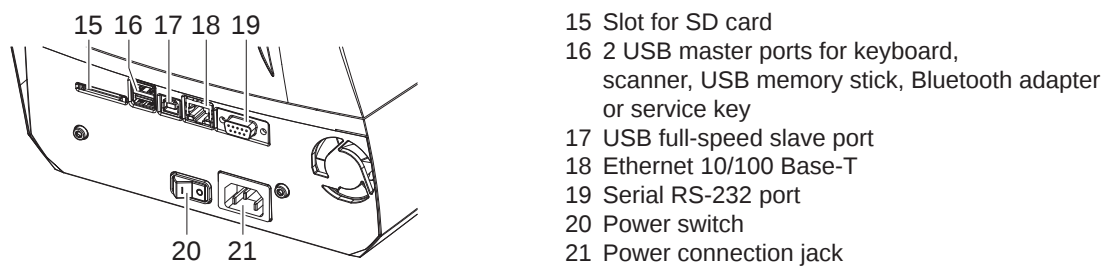
Figure 3 Connections
